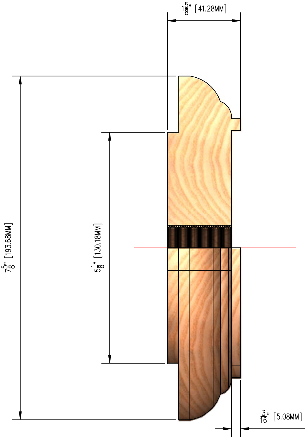
Clock body mandrel
