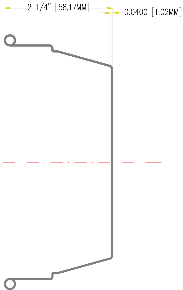
Spun Part 1100-O Aluminim 0.040" Thk
